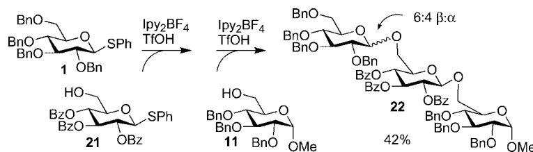
Scheme 1. One-pot glycosylation reaction.
